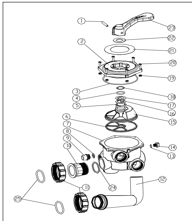
Spare Parts List for 1.5" Side Mounted Multiport Valves
